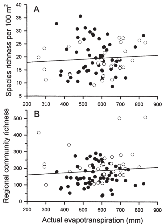
Fig. 2. Relationship between AET and (A) Mean local species richness, standardized at a grain of 100 m 2 , and (B) Regional community richness. Closed symbols indicate non-transitional regions, open symbols indicate transitional regions. Simple regressions are shown here for illustrative purposes only. See Table 2 for statistics of the multiple regression models.
