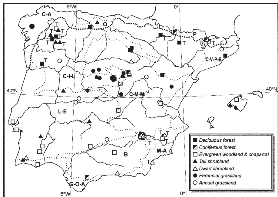
Fig. 1. Locations of the 93 data sets in the Iberian Peninsula and the Balearic Islands. The dashed lines indicate borders between biogeographical provinces. The bold dashed line is the border between the Atlantic and the Mediterranean climatic zones. T indicates a transitional data set (see text), some T signs indicate more than one data set.
