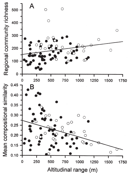
Fig. 3. Relationship between altitudinal range and (A) Regional community richness and (B) compositional mean similarity. Closed symbols indicate non-transitional regions, open symbols indicate transitional regions. Simple regressions are shown here for illustrative purposes only. See Table 2 for statistics of the multiple regression models.
